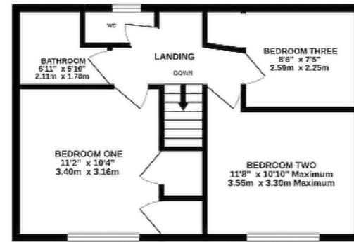
1ST FLOOR 431 sq.ft. (40.0 sq.m.) approx.
